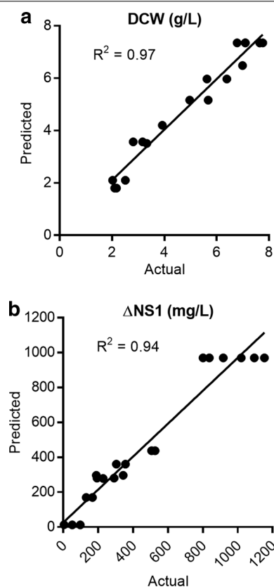
Fig. 2 Predicted vs actual plots for biomass and \Delta NS1. Linear regression plot for the predicted and actual responses for a biomass formation (g/L DCW) and b \Delta NS1 (mg/L) obtained in soluble fraction of cell extracts
