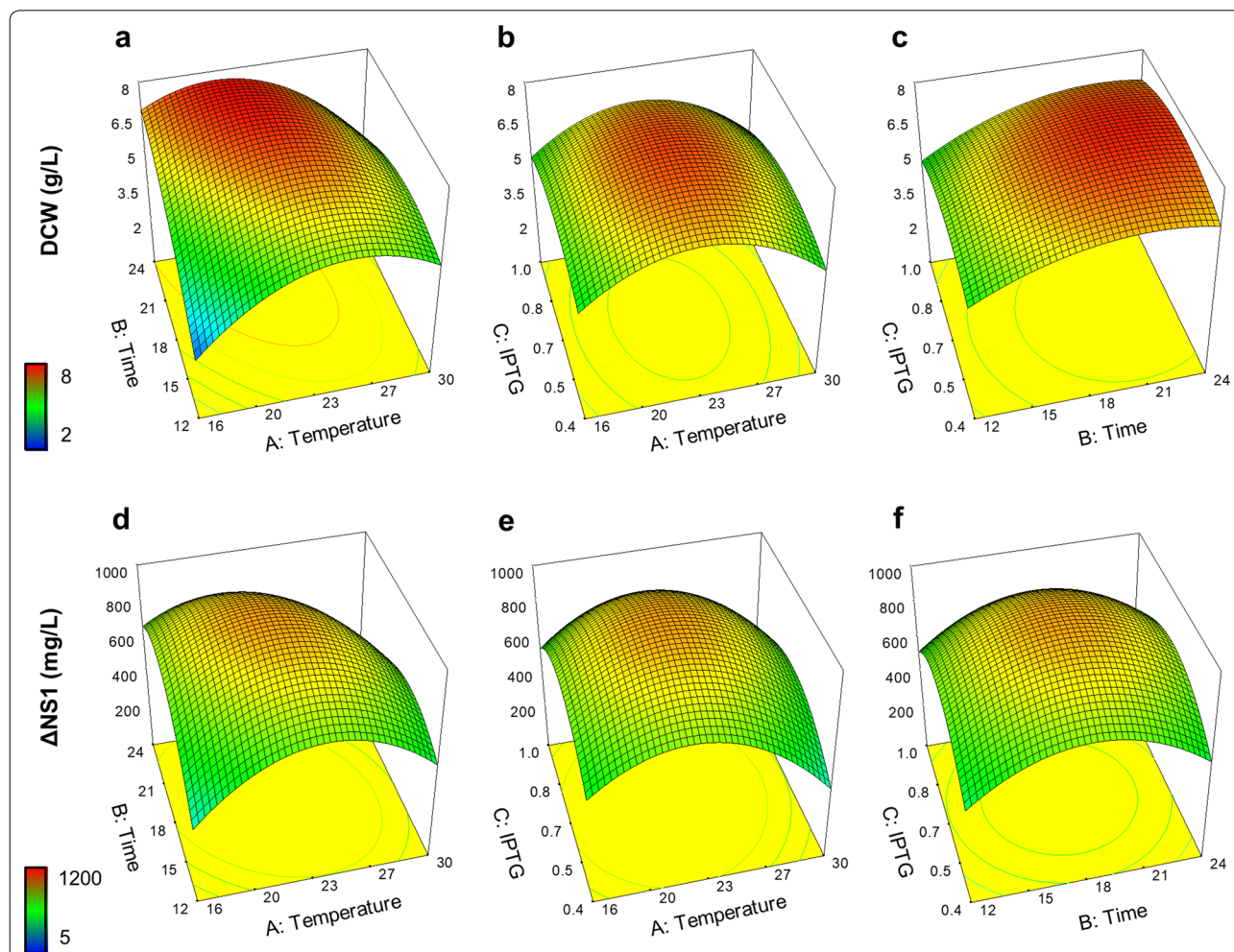
Fig. 1 Response surface plots for biomass and production of soluble \Delta NS1 as a function of time, temperature of induction and IPTG concentration. The model generated by the CCD for a–c biomass concentration measured as dry cell weight (DCW g/L) and d–f production of \Delta NS1 the soluble fraction of cell extracts (mg/L). The temperature range was 16–30 °C, time between 12 and 24 h of induction and IPTG concentration between 0.4 and 1.0 mM. Color-coding indicates high (red) and low (blue) responses
